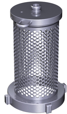
FBSD60—Separated (For Barrel Strainer Applications)
