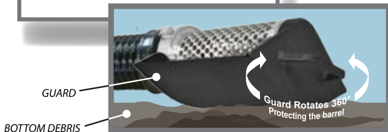
GUARD IN POSITION PROTECTING THE BARREL STRAINER
